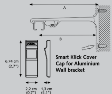
Aluminium Wall bracket single A) 10 cm (4") B) 8,8 cm (3,5")
