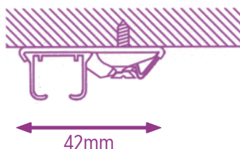
Ceiling Bracket
