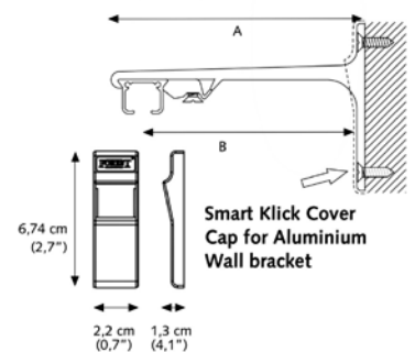
Aluminium Wall bracket single A) 10 cm (4") B) 8,8 cm (3,5")
