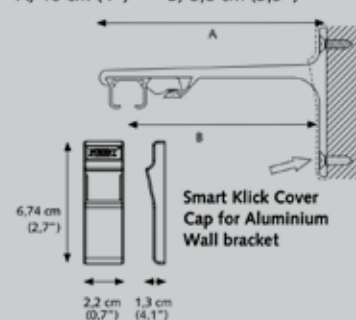
Aluminium Wall bracket single
